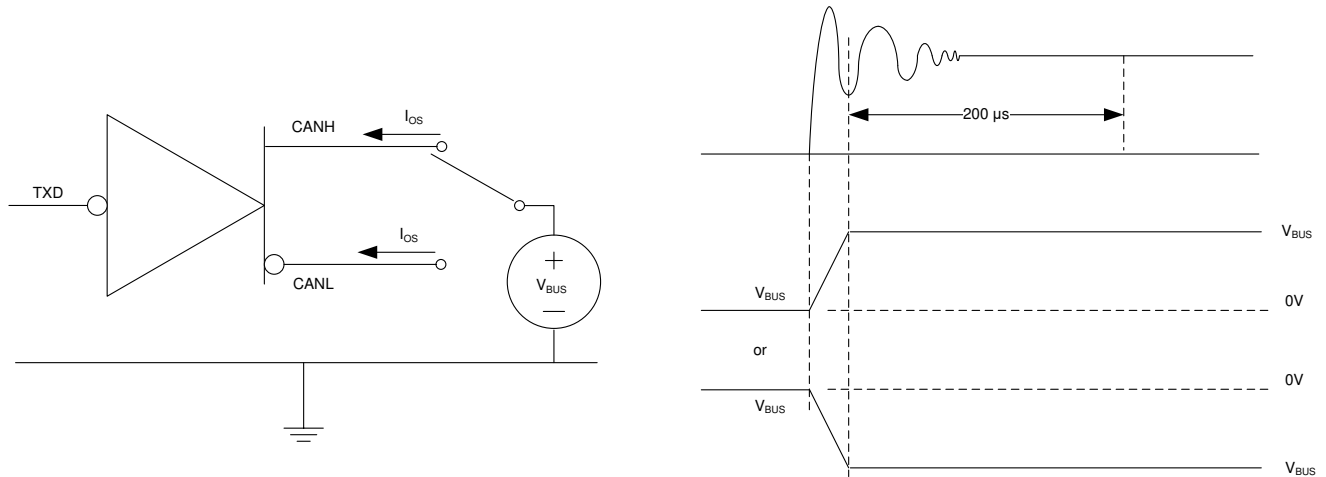
图 11. Driver Short-Circuit Current Test and Measurement
