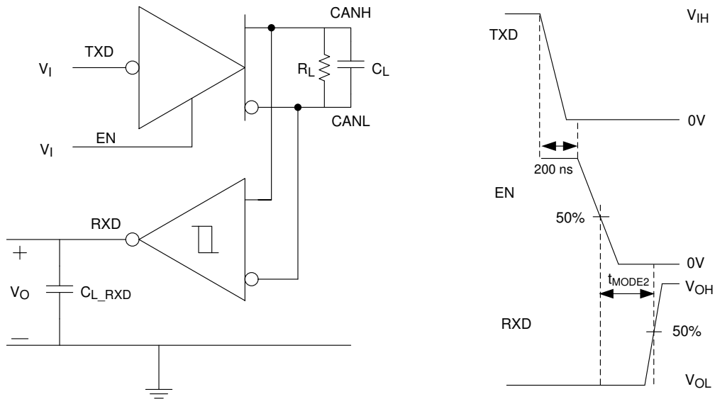
图 9. t_{MODE2} Test Circuit and Measurement, Normal Mode to Silent Mode
