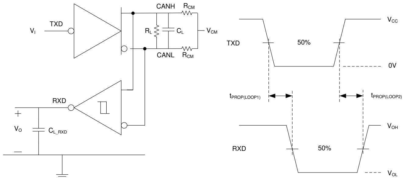
图 10. t_{\text{PROP(LOOP)}} Test Circuit and Measurement
