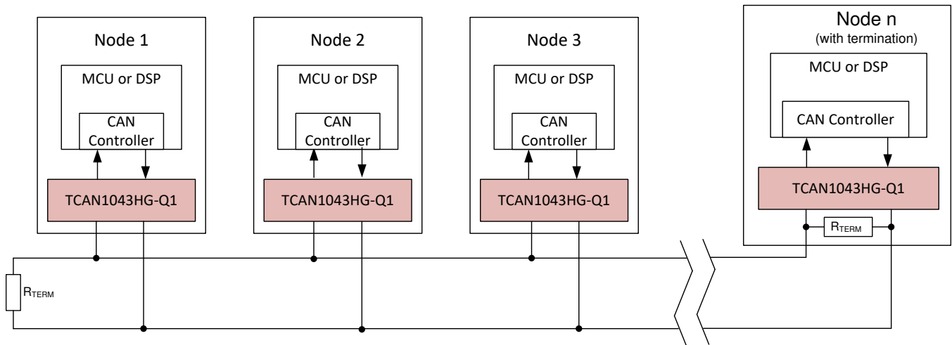
图 28. Typical CAN Bus Application
