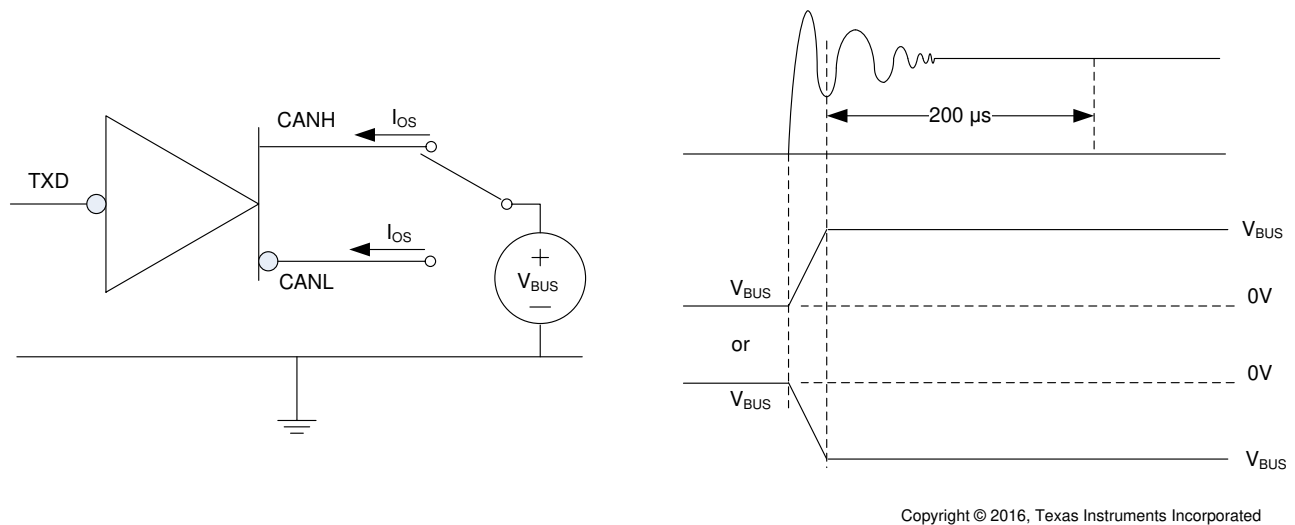
图 14. Driver Short-Circuit Current Test and Measurement
