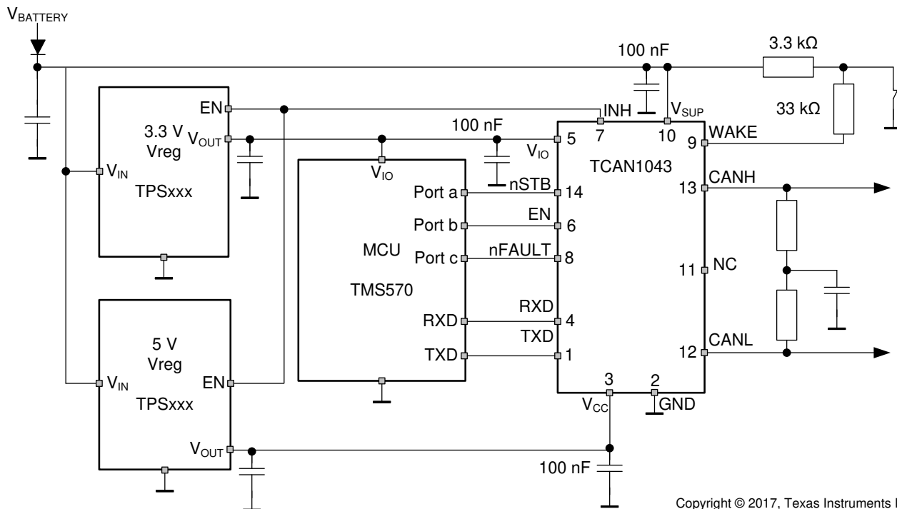
图 27. Typical CAN Bus Application Using TCAN1043xx-Q1 with 3.3 V \mu C
