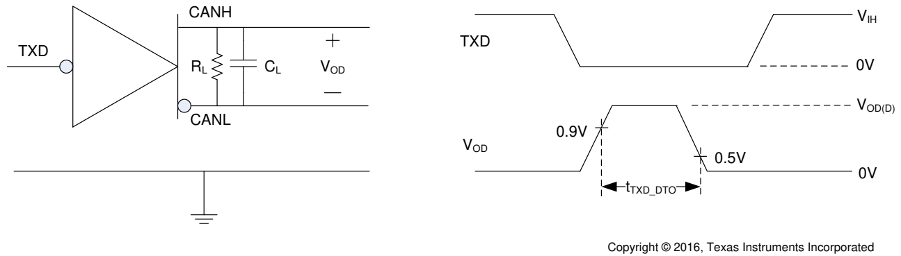
图 13. TXD Dominant Timeout Test Circuit and Measurement
