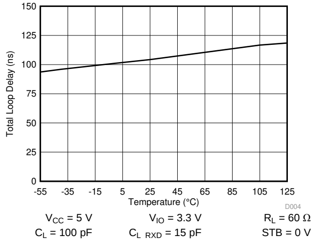
图 4. Total Loop Delay over Temperature
