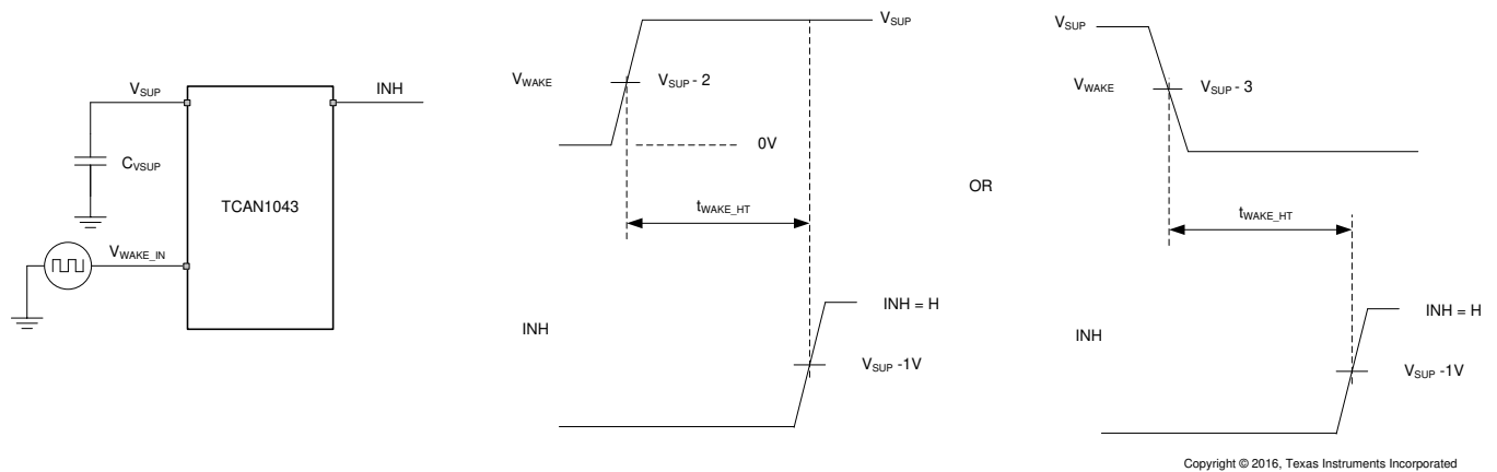
图 16. t_{\text{Wake\_HT}} While Monitoring INH Output
