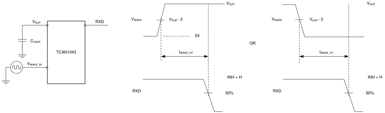
图 17. t_{WAKE\_HT} While Monitoring RXD Output
