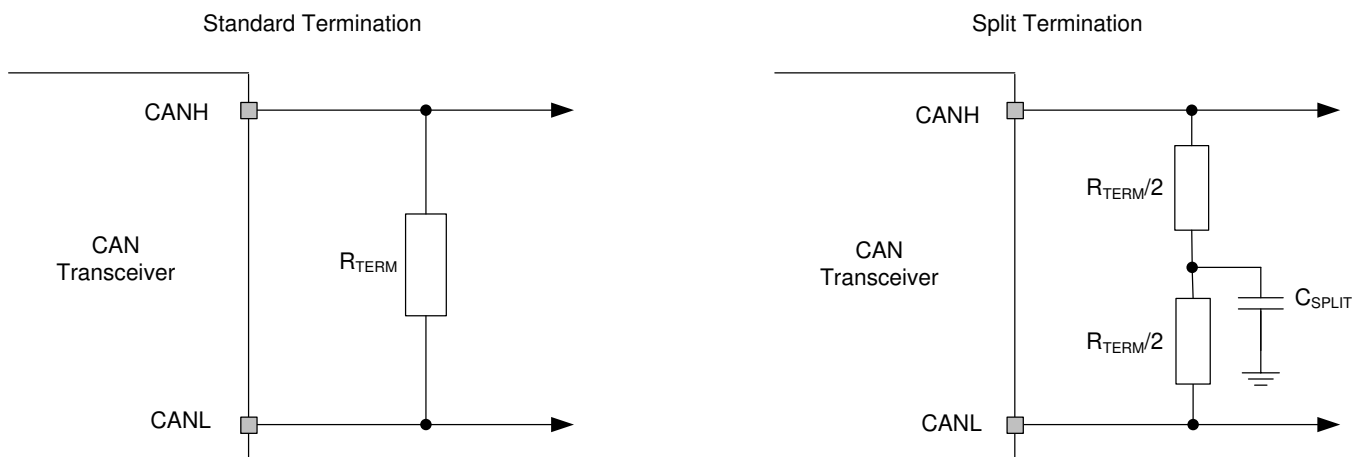
图 29. CAN Bus Termination Concepts
