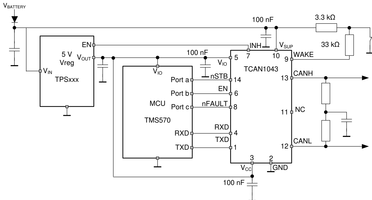
图 26. Typical CAN Bus Application Using TCAN1043xx-Q1 with 5 V \mu C
