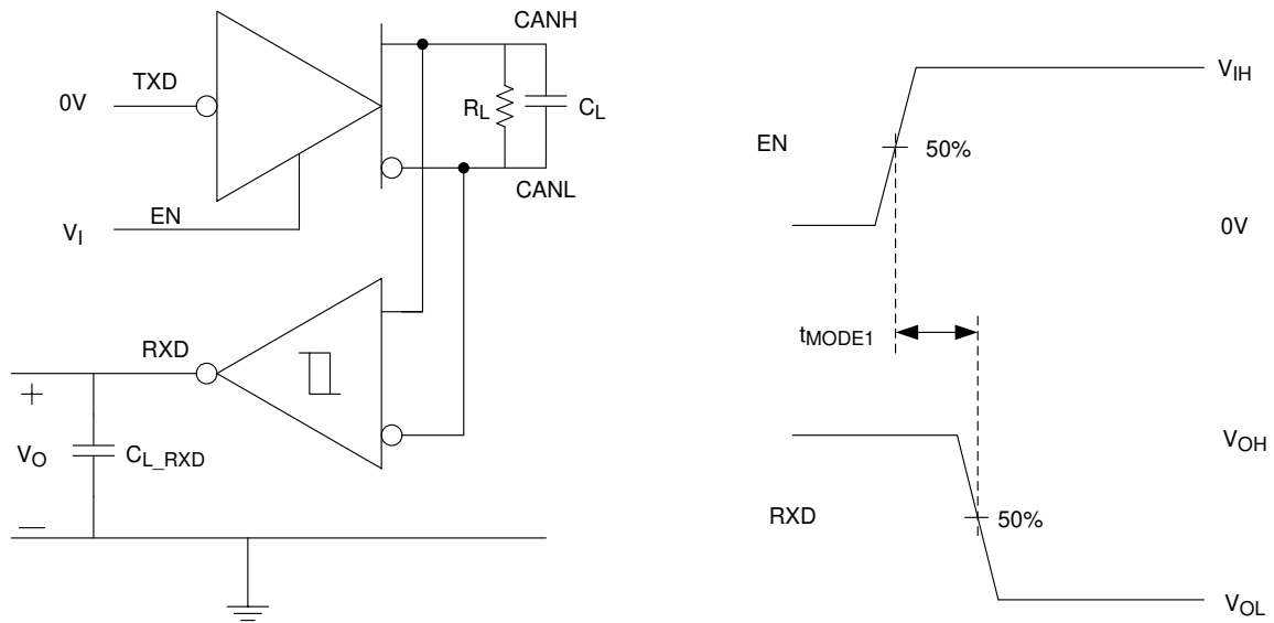
图 8. t_{MODE1} Test Circuit and Measurement, Silent Mode to Normal Mode
