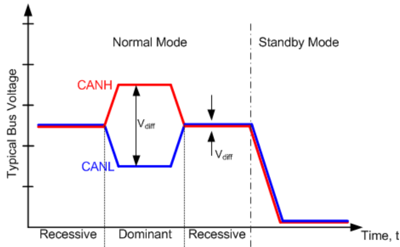
图 19. Bus States (Physical Bit Representation)
