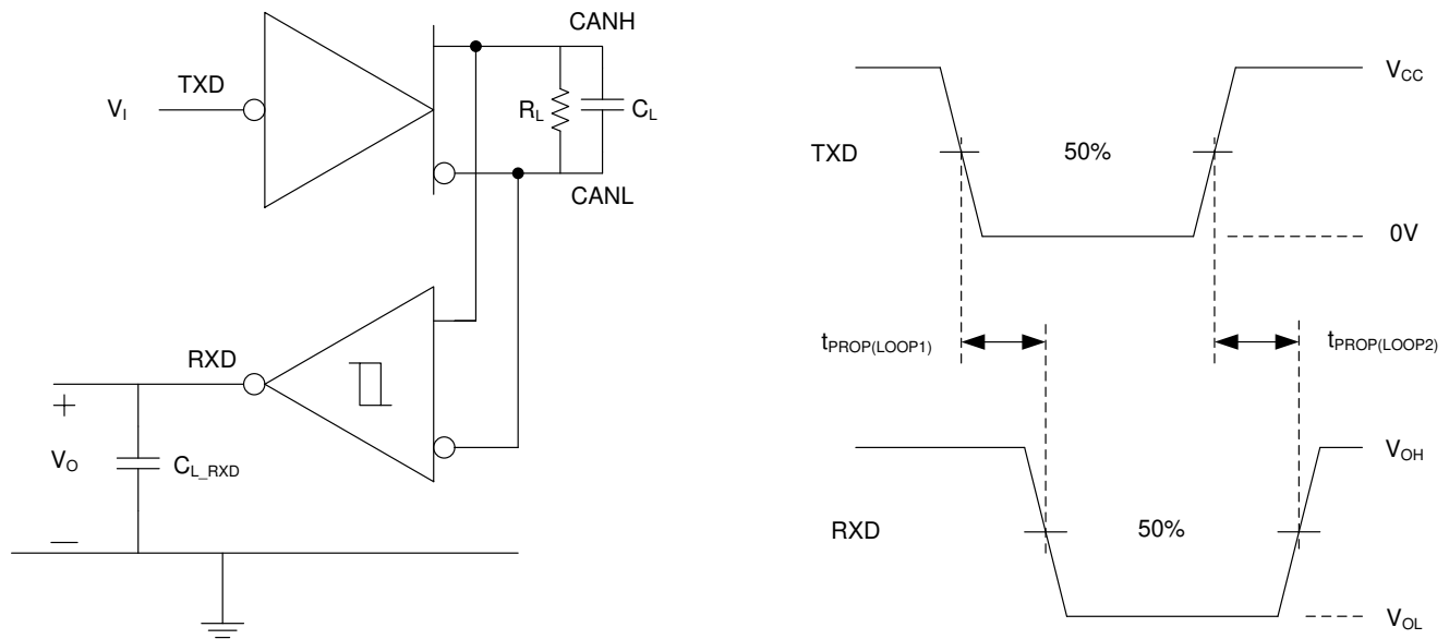
图 10. t_{\text{PROP(LOOP)}} Test Circuit and Measurement
