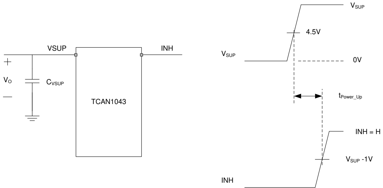
图 15. t_{\text{Power\_Up}} Timing Measurement
