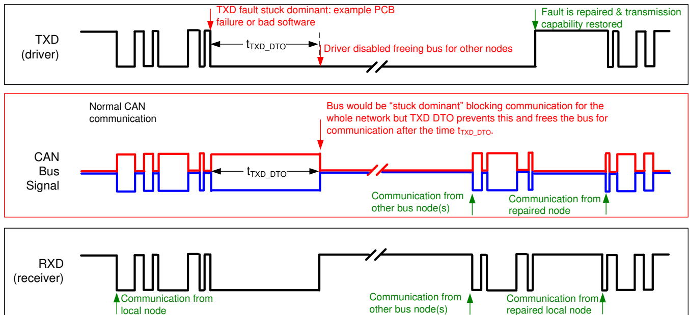
图 18. Example Timing Diagram for TXD DTO
