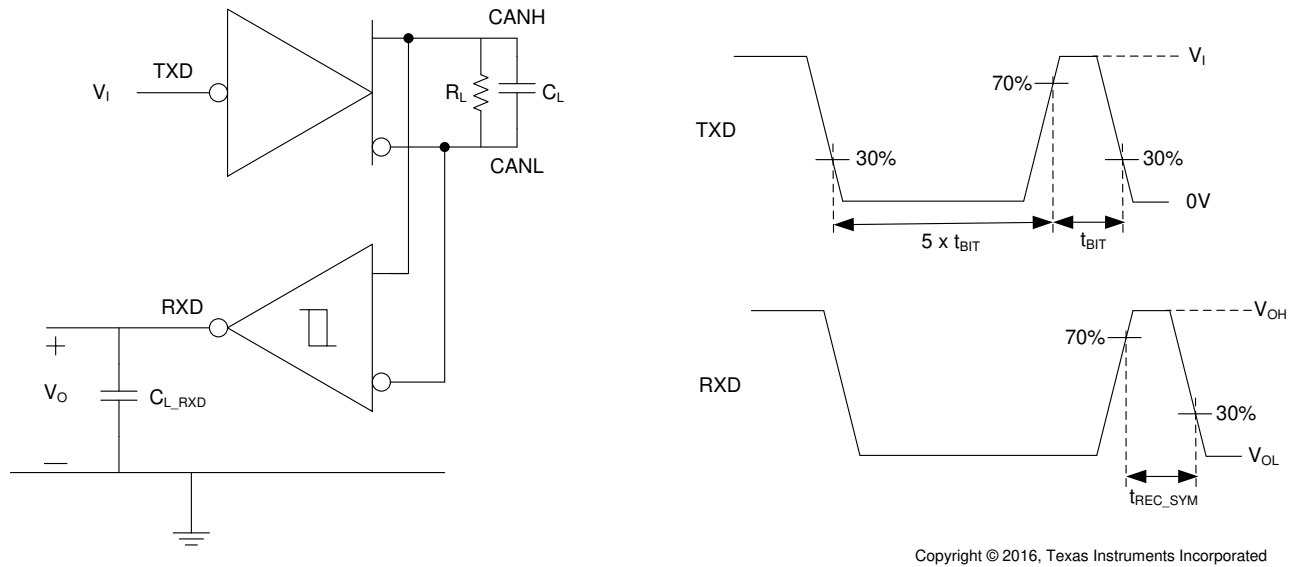
图 12. Loop Delay Symmetry Test Circuit and Measurement
