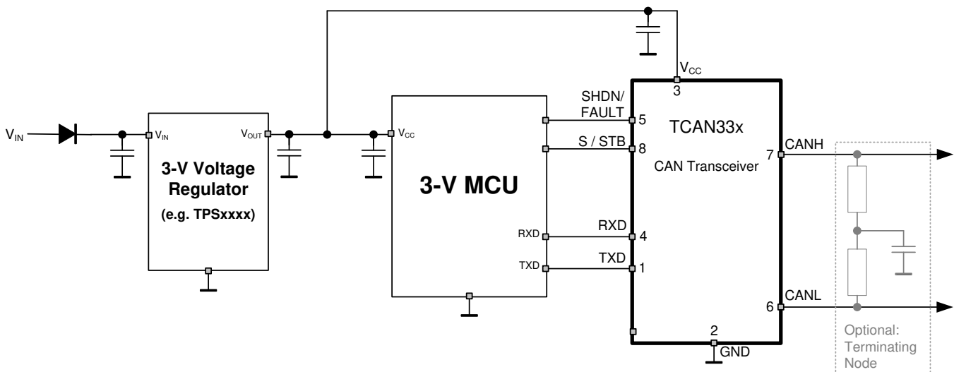
Figure 34. Typical 3.3-V Application
