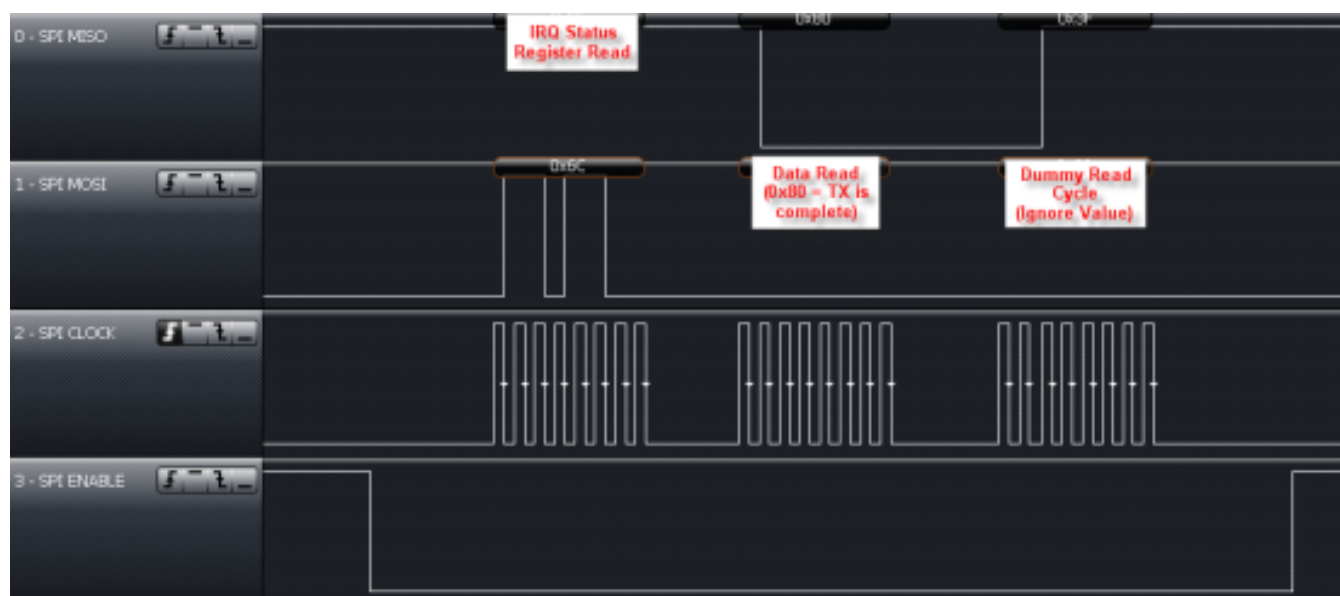
图 6-18. Example of Dummy Read Using SPI With SS
