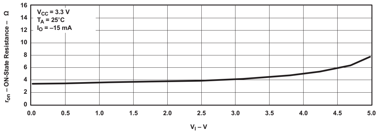
Figure 1. Typical r_{on} vs V_I
