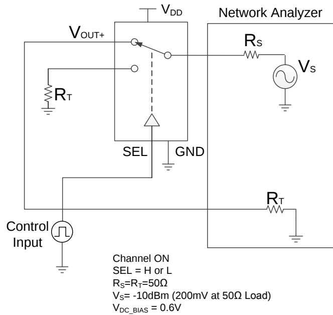
图 17. Bandwidth Measurement
