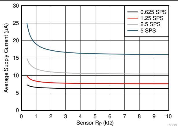
Figure 6-4. Supply Current vs Sensor R_P for Low Power Mode. Sensor Frequency = 3.6 MHz.
