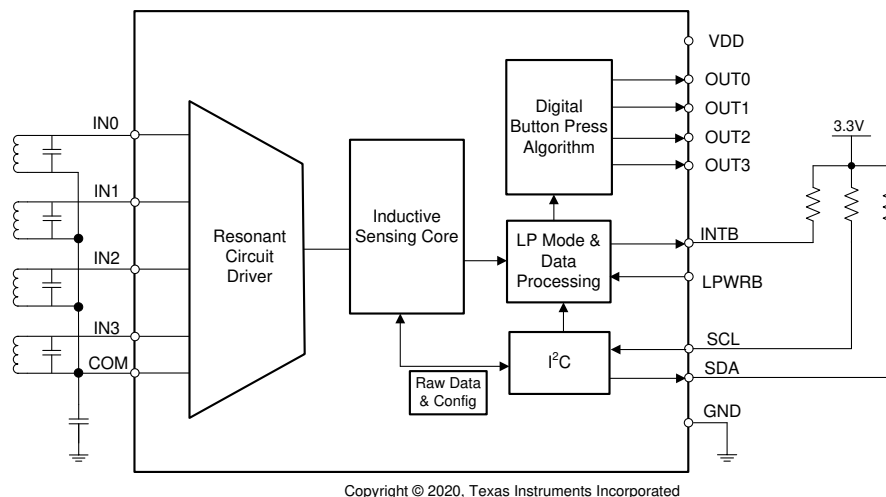
Figure 7-1. Block Diagram of LDC3114-Q1
