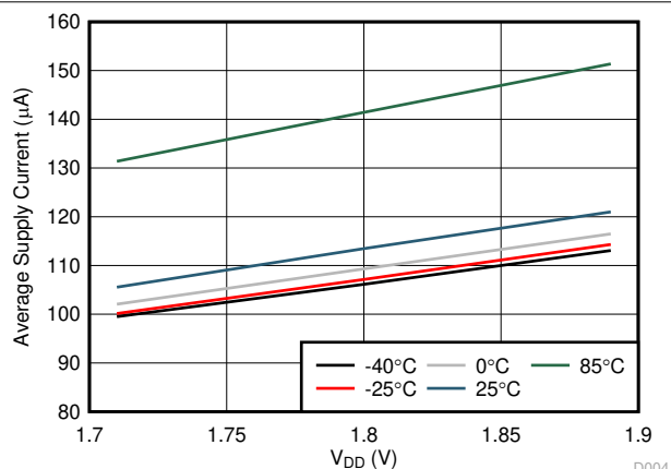
Figure 6-6. Supply Current vs. V_{DD} . Sensor R_P = 650\ \Omega , Scan Rate = 40 SPS.
