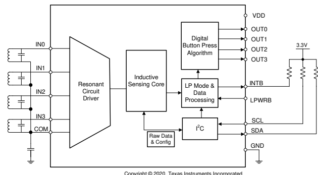
LDC3114-Q1 Simplified Schematic
