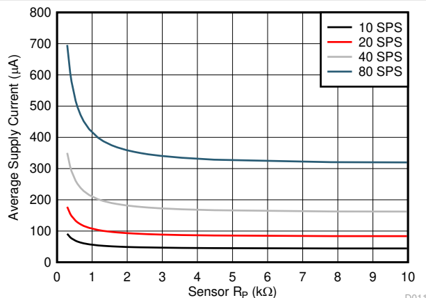
Figure 6-3. Supply Current vs Sensor R_P for Normal Power Mode. Sensor Frequency = 3.6 MHz. Two Channels Enabled.
