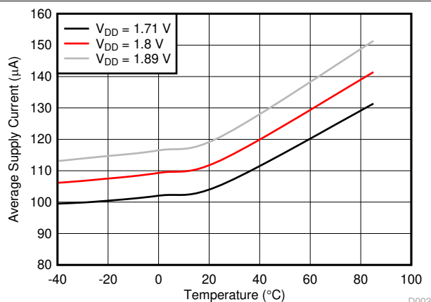
Figure 6-5. Supply Current vs Temperature. Sensor R_P = 650\ \Omega , Scan Rate = 40 SPS.
