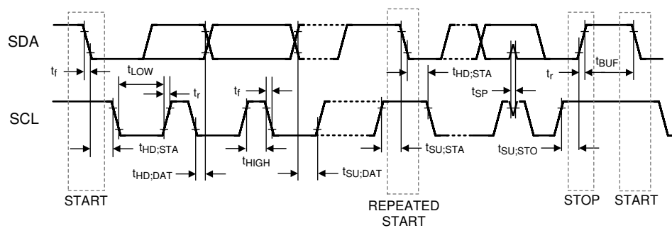
Figure 6-1. I 2 C Timing Diagram
