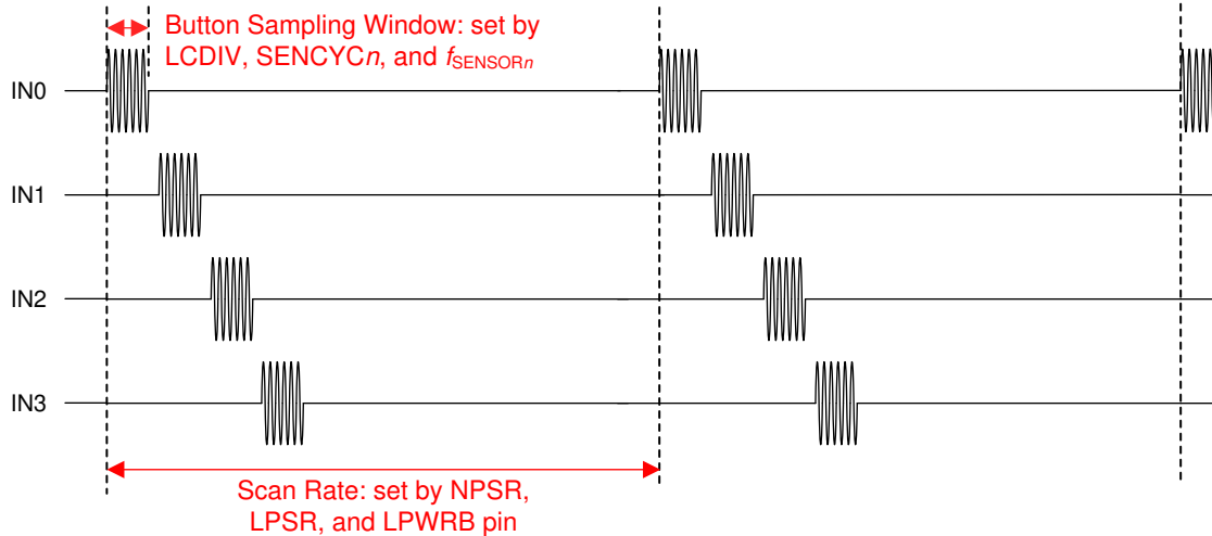
Figure 8-6. Configurable Scan Rate and Button Sampling Window
