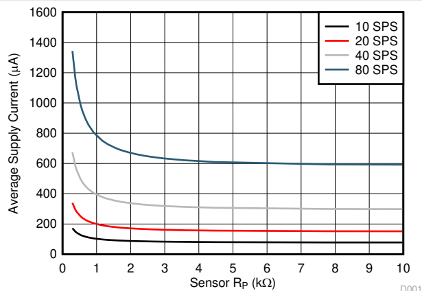
Figure 6-2. Supply Current vs Sensor R_P for Normal Power Mode. Sensor Frequency = 3.6 MHz. Four Channels Enabled.
