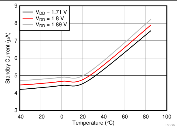
Figure 6-7. Standby Current vs. Temperature
