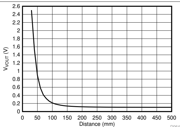
图 69. Analog Output Voltage of the DRV425-Q1 vs Distance to the Magnet
