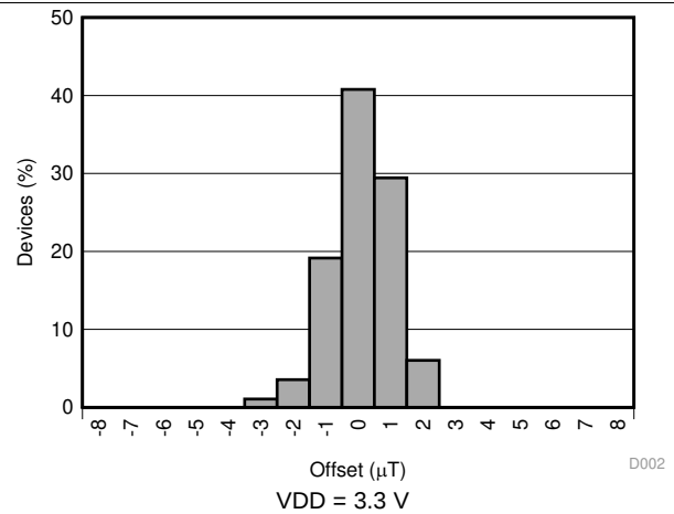
图 2. Fluxgate Sensor Front-End Offset Histogram
