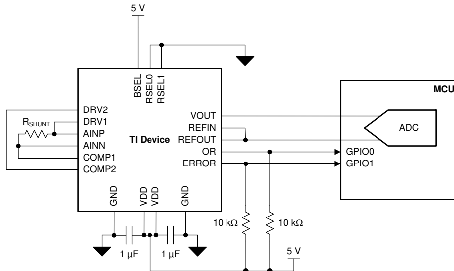
图 67. Linear-Position Sensing
