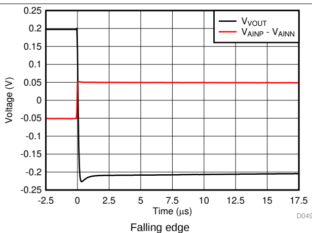
图 42. Shunt-Sense Amplifier Small-Signal Settling Time
