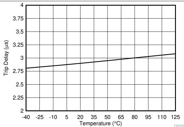
图 38. \overline{\text{OR}} Pin Trip Delay vs Temperature
