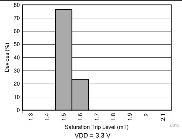
图 14. Fluxgate Sensor Saturation ( \overline{\text{ERROR}} Pin) Trip Level Histogram
