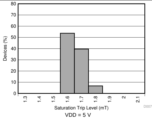
图 13. Fluxgate Sensor Saturation ( \overline{\text{ERROR}} Pin) Trip Level Histogram
