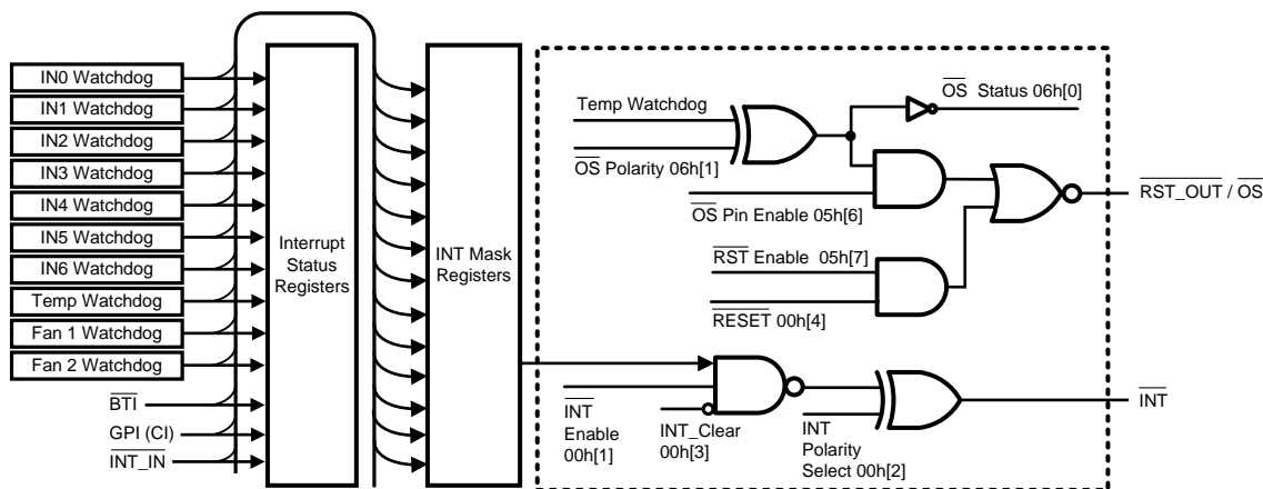
Figure 22. Interrupt Structure
