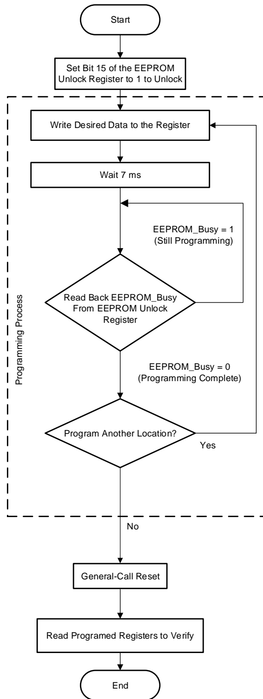
图 20. EEPROM Programming Sequence
