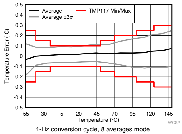
图 3. YBG Package Temperature Error vs Temperature
