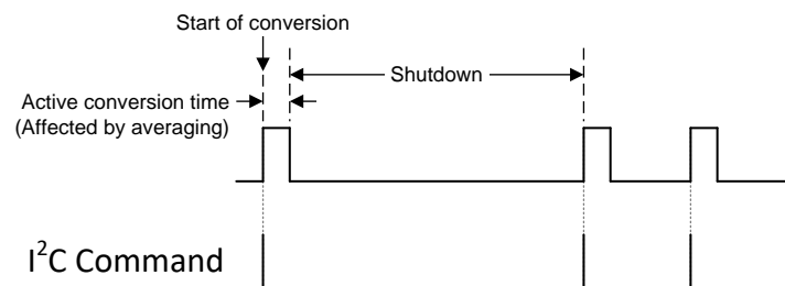
图 17. One-Shot Timing Diagram With AVG[1:0] = 00
