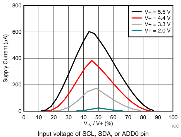
图 13. Supply Current vs Input Cell Voltage
