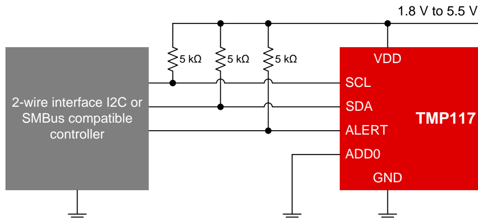
图 36. Typical Connections
