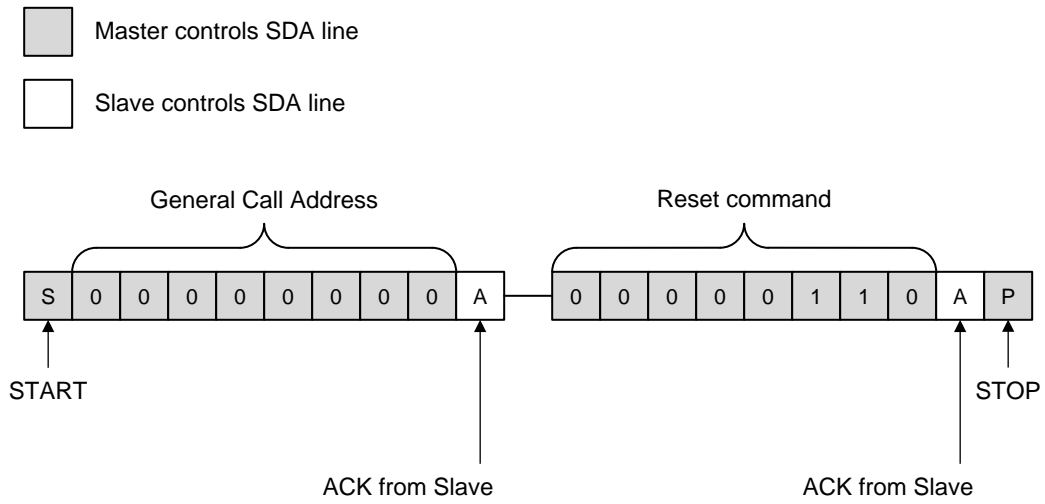
图 25. General-Call Reset Command Timing Diagram
