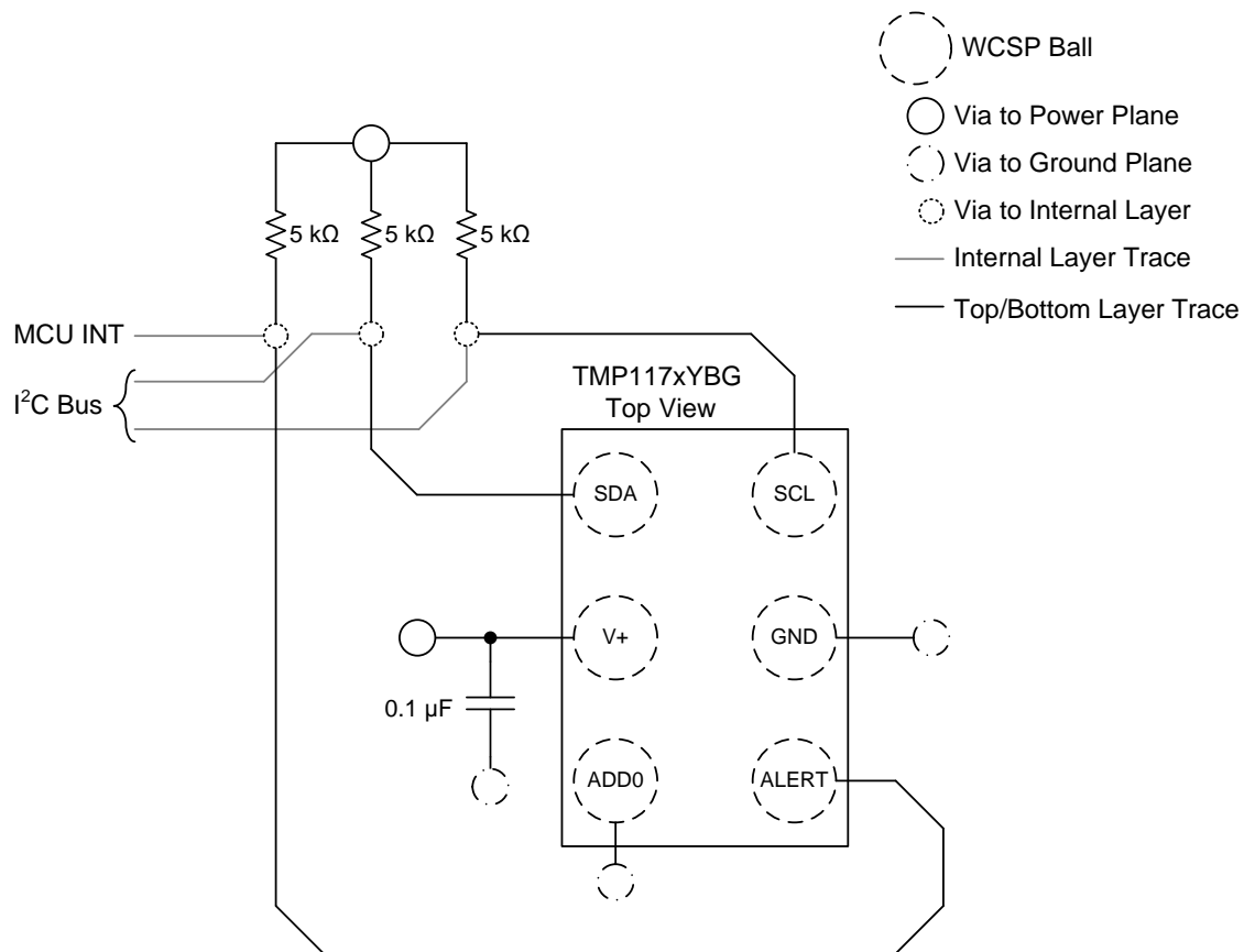
图 41. YBG Layout Recommendation
