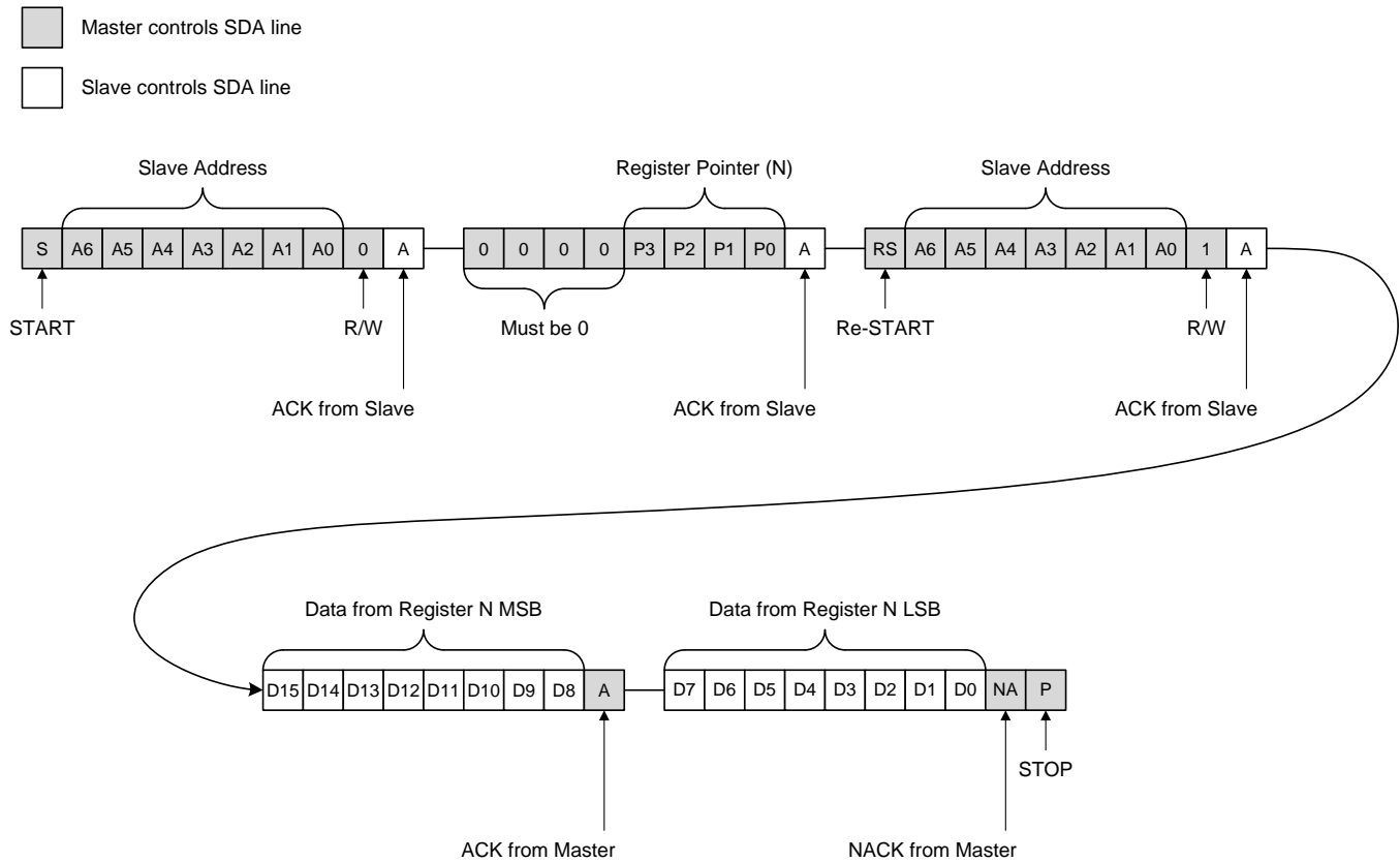
图 23. Read Word Command Timing Diagram
