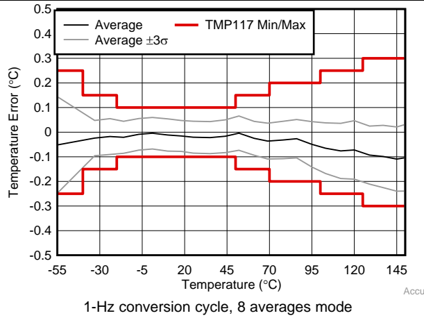
图 2. DRV Package Temperature Error vs Temperature
