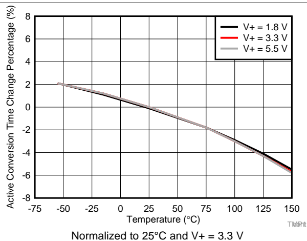
图 11. Active Conversion Time vs Temperature
