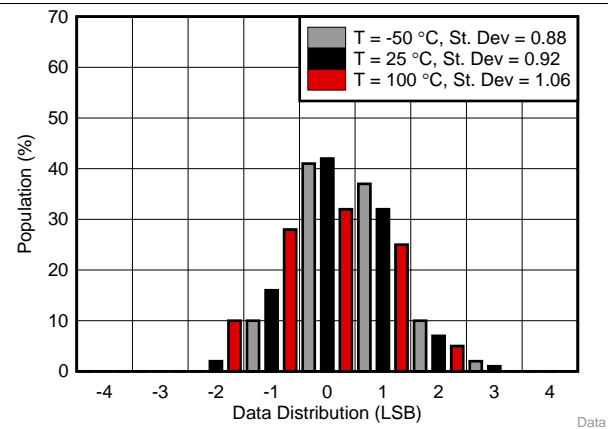
图 6. Data Reading Distribution Over Temperature (No Averaging, V_+ = 3.3\text{ V} )
