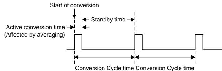
图 16. Conversion Cycle Timing Diagram
