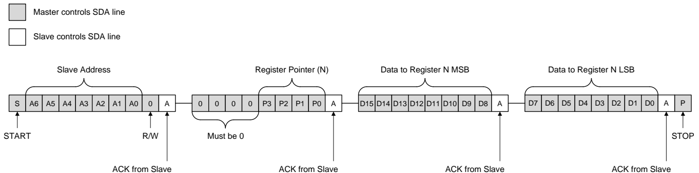
图 22. Write Word Command Timing Diagram
