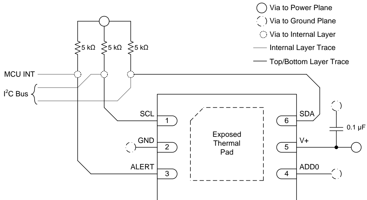
图 40. DRV Layout Recommendation
