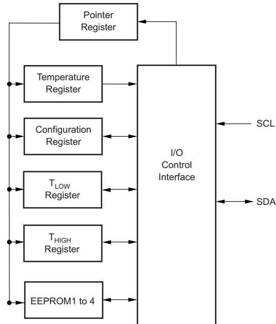
图 21. Internal Register Structures
