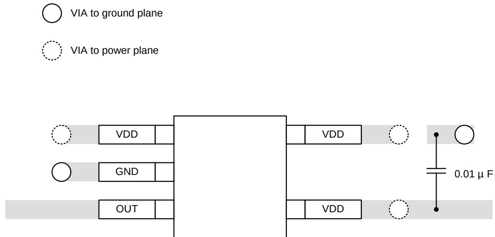
Figure 19. SC70 Package Recommended Layout
