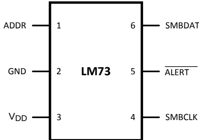
Pin Functions
