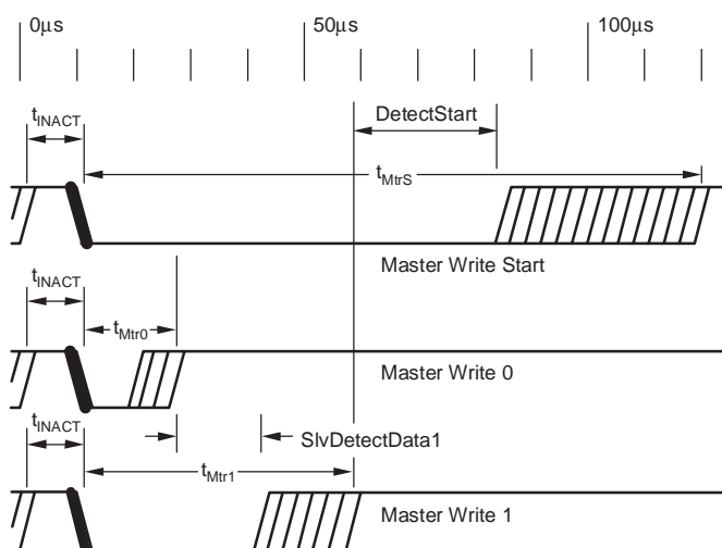
1a: Master Write timing and slave detection of the data placed on the SWD bus by the master.
